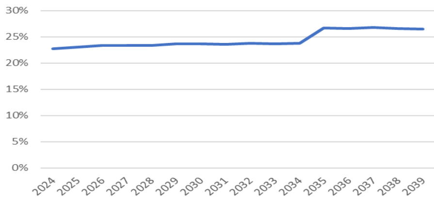
Reserve Margin (%)
