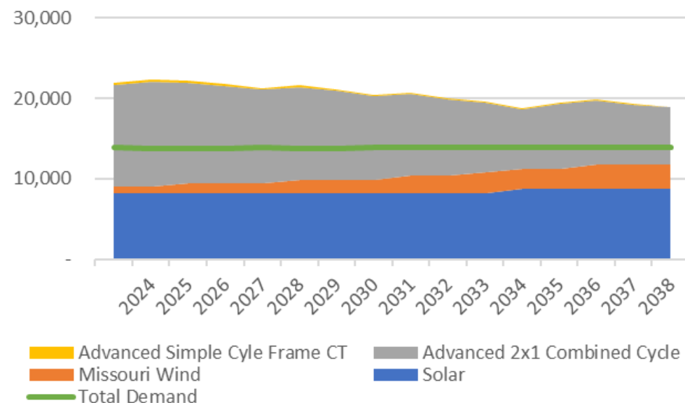
Total Generation Vs. Total Demand (GWh)
